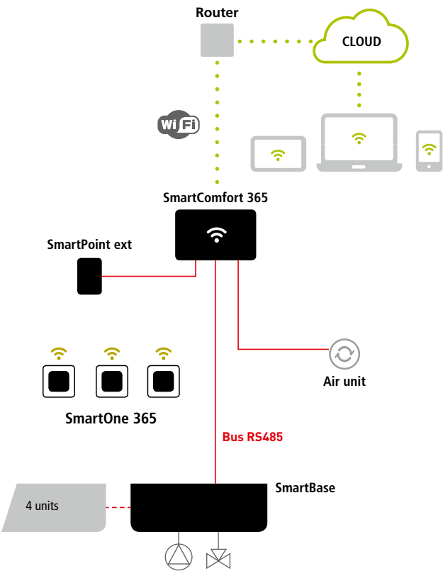
SMARTCOMFORT 365 + SMARTONE 365 AS A ROOM SENSORS
