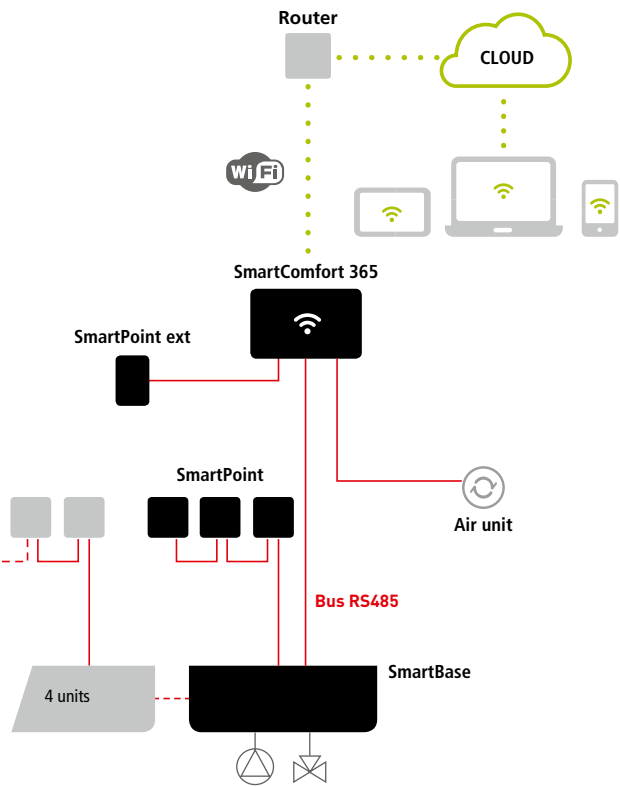
SMARTCOMFORT 365 REGULATION SYSTEM: BUS CONNECTION
