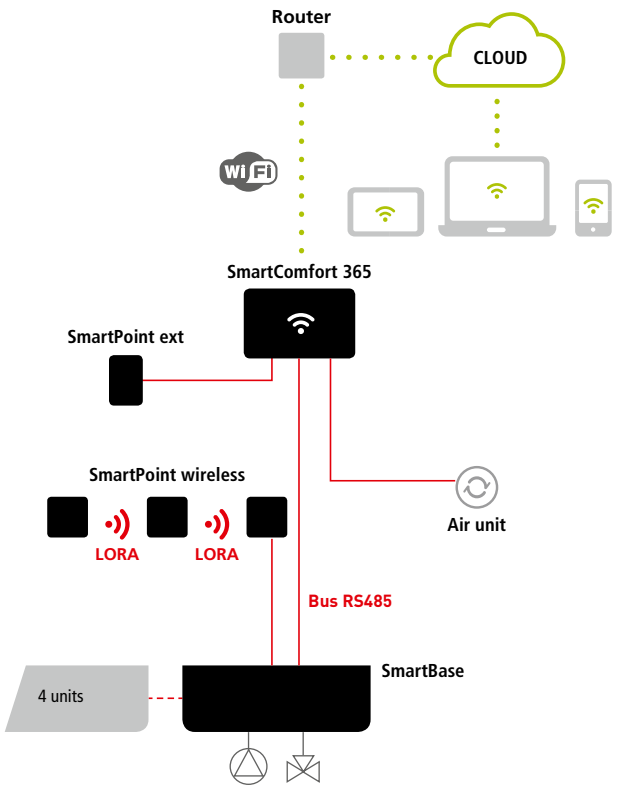
SMARTCOMFORT 365 REGULATION SYSTEM: WIRELESS CONNECTION
