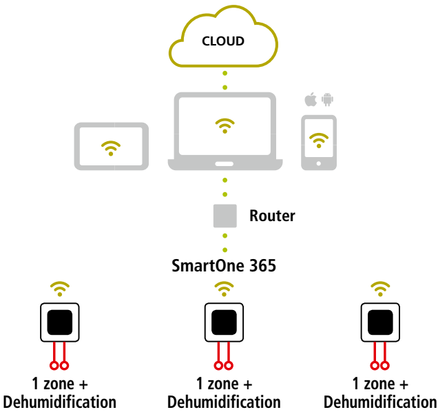
SMARTONE 365 REGULATION SYSTEM: HEATING/COOLING/DEHUMIDIFICATION
